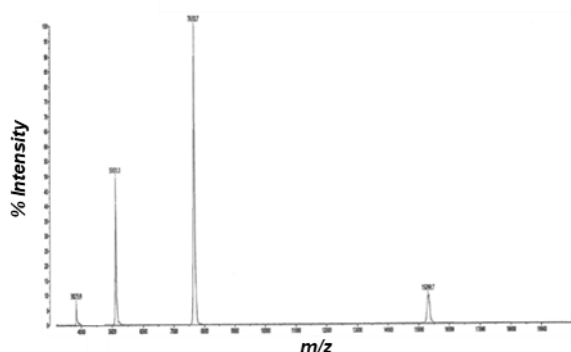
Figure 3: Mass spectrometry analysis of Synthetic H3K9Ac histone. Confirming the expected mass (15,299 Da) matches the observed mass (15,299.7 Da).
